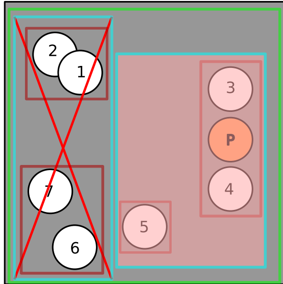
Figure 183: Querying an AABB-tree (2/3)
